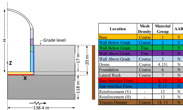
(d) Model and accompanying material groups Figure 15: Geometry and model idealization
