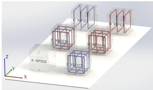
Figure 2: 14" \times 14" \times 14" blocks with various reinforcements
