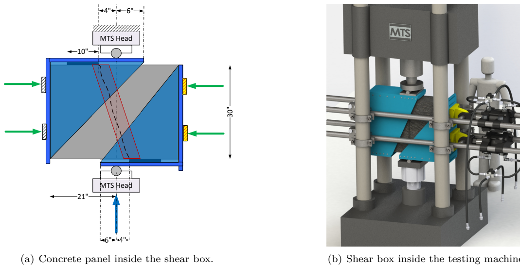
Figure 6: Experimental Set-up
