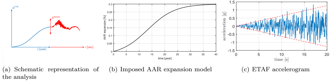
Figure 16: Loads imposed on the NCVS analysis
