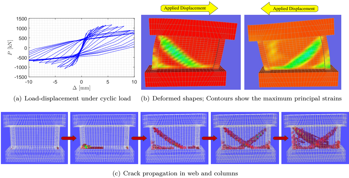
Figure 13: Structural response of shear wall under cyclic displacement (without ASR)
