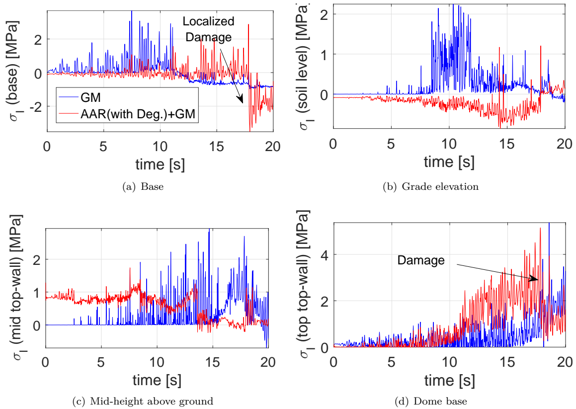
Figure 19: Principal stress-time histories from the seismic analysis
