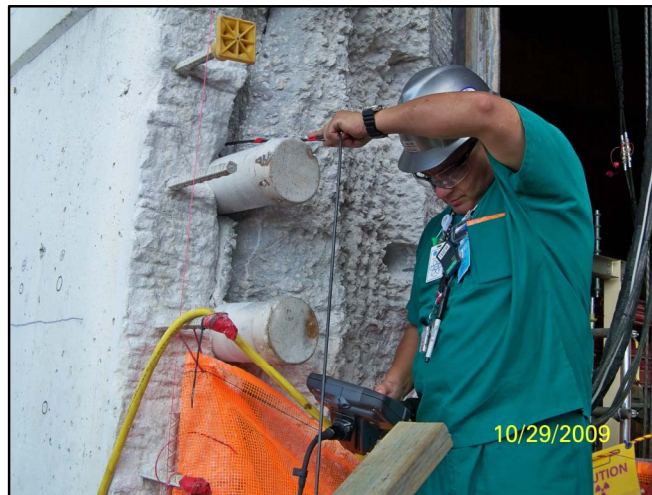
Figure 4: 5" tendon conduits (Progress Energy Florida (ML102861026), 2009)
