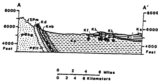
Figure 4. Generalized NW-SE geologic cross section across Boulder. Location shown as A-A' on Figure 3. See Figure 3 for explanation of symbols. Adapted from Hall and others (1980).
