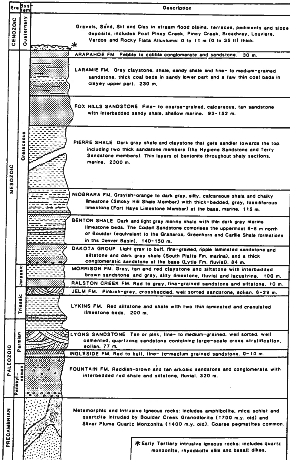
Figure 6. Stratigraphic column for Boulder County. Adapted from Malde, (1955), Wells (1967), Wrucke and Wilson (1967), and Madole (1973).
