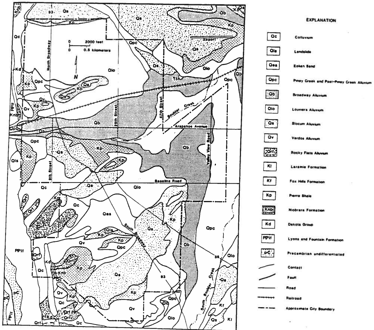
Figure 5. Geologic map of the City of Boulder. Adapted from Spencer (1961), Wrucke and Wilson (1967), Wells (1967), Trimble (1975), Colton (1978), and Trimble and Machette (1979).
